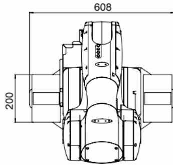
(c) 俯视图
