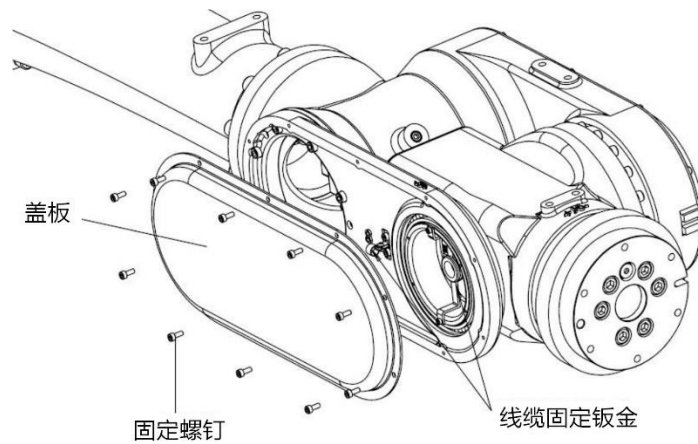
图 12-7 AIR50-2260/AIR80-2260/AIR50-2700/AIR80-2560 腕部内部线缆
