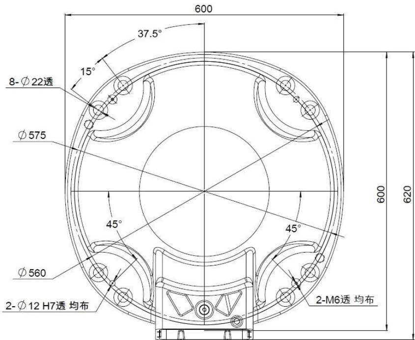
图 4-1 AIR50-2260/AIR80-2260/AIR35-2700/AIR20-3100 操作机基座接口尺寸
