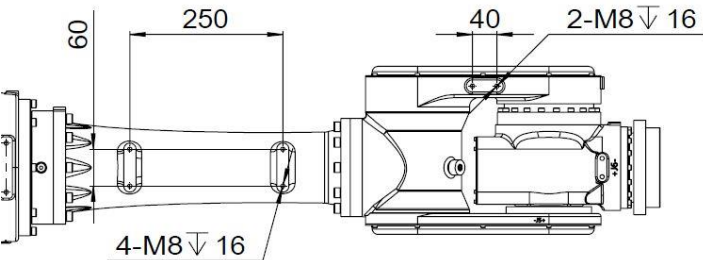
图 7-20 AIR50-2260/AIR80-2260/AIR50-2700/AIR80-2560 操作机小臂接口尺寸图
