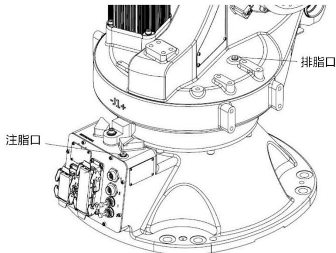
图 12-11 AIR50-2260/AIR80-2260/AIR35-2700/AIR20-3100 更换 J1 轴减速器润滑脂
