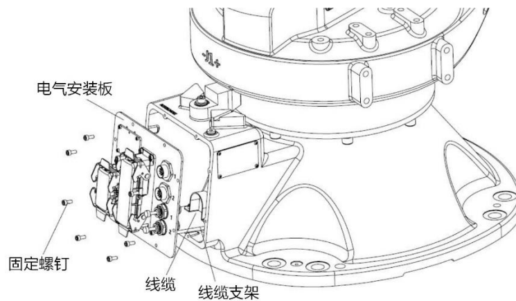
图 12-4 AIR50-2260/AIR80-2260/AIR35-2700/AIR20-3100 底座内部线缆
