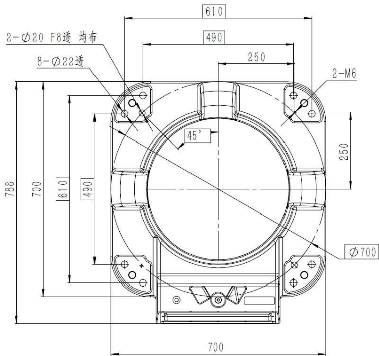
图 4-2 AIR50-2700/AIR80-2560 操作机基座接口尺寸
