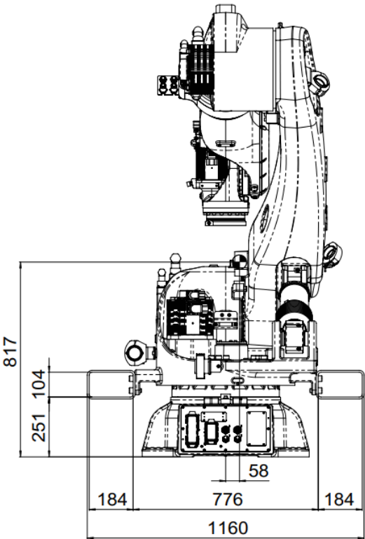
图 9-4 AIR280-2700/AIR130-2700/AIR170-2700/AIR220-2700 搬运时操作机尺寸
