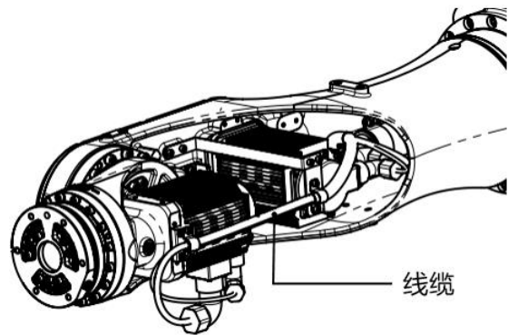
图 12-6 AIR220-3100/AIR130-3100/AIR170-3100 腕部内部线缆
