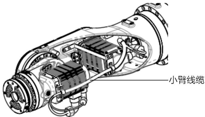
图 12-5 AIR280-2700/AIR130-2700/AIR170-2700/AIR220-2700 腕部内部线缆
